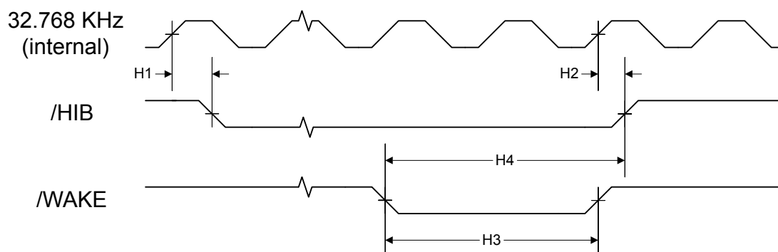
Figure 21-10. Hibernation Module Timing
