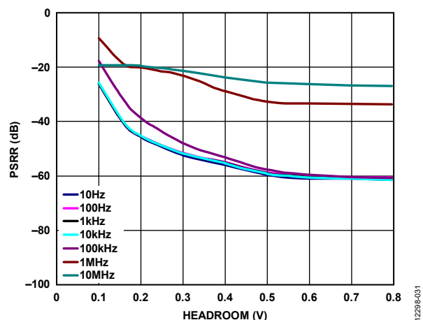
Figure 31. Power Supply Rejection Ratio (PSRR) vs. Headroom, V_{OUT} = 3\text{ V} , 1 A Load Current, Different Frequencies
