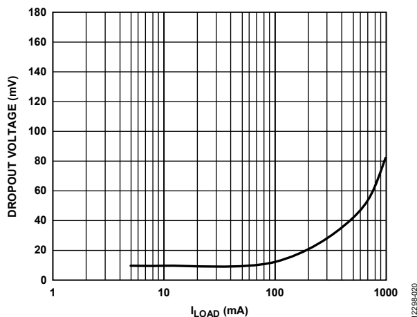
Figure 20. Dropout Voltage vs. Load Current ( I_{LOAD} ), V_{OUT} = 3\text{ V}
