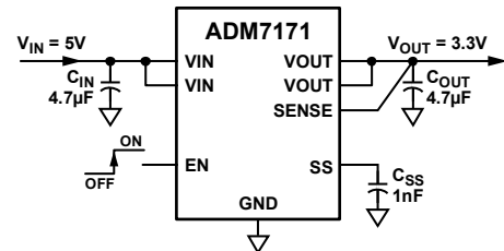
Figure 1. ADM7171 with Fixed Output Voltage, 3.3 V
