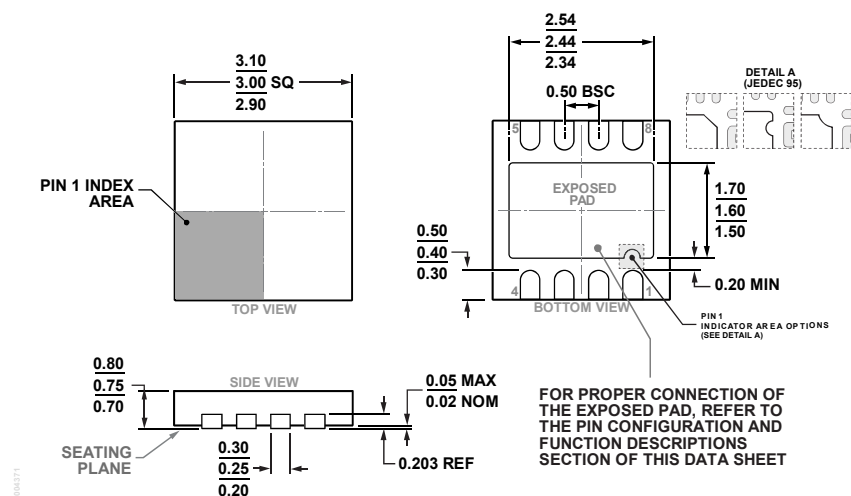
Figure 70. 8-Lead Lead Frame Chip Scale Package [LFCSP] 3 mm × 3 mm Body and 0.75 mm Package Height (CP-8-21)
