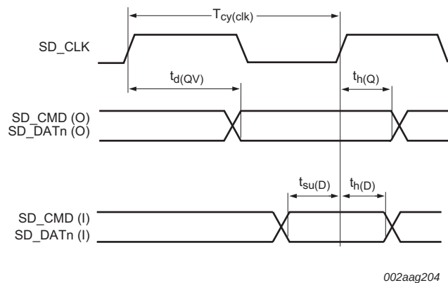
Fig 37. SD/MMC timing
