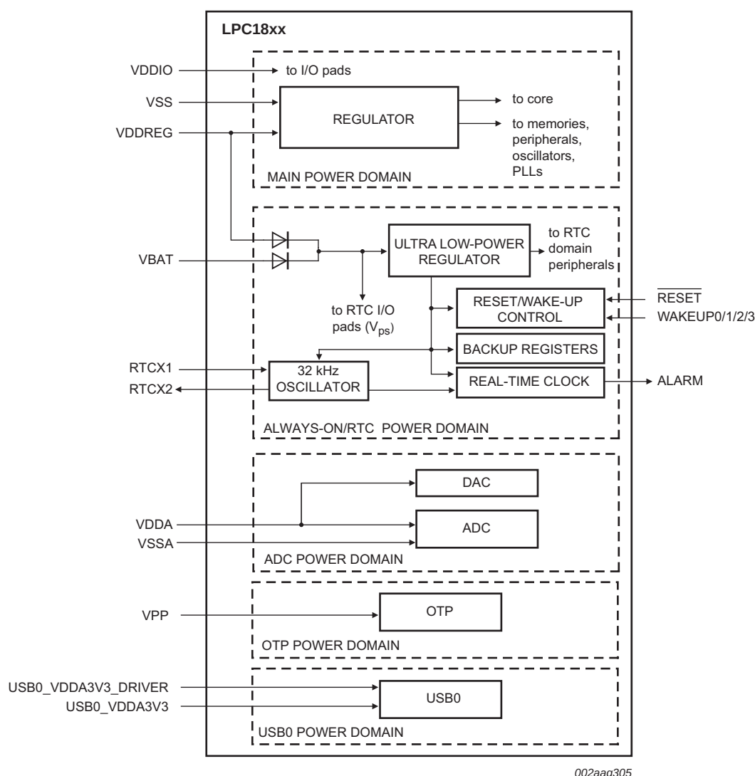
Fig 9. LPC18S50/S30/S10 power domains
