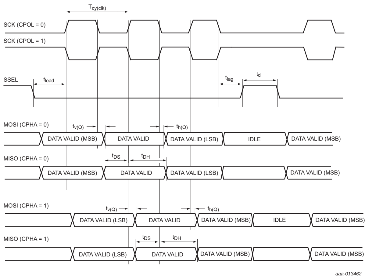
Fig 30. SSP master mode timing (SPI mode)
