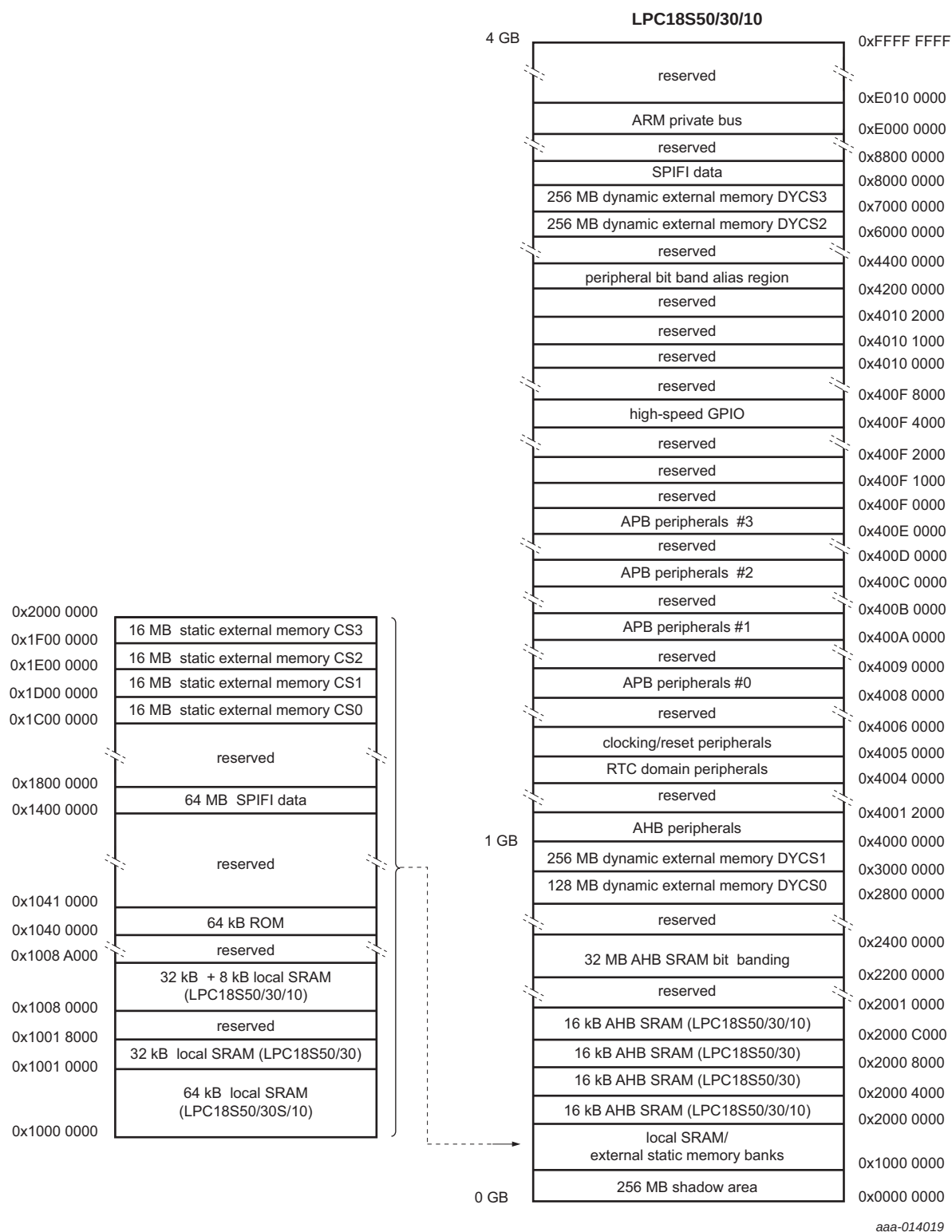
Fig 7. LPC18S50/S30/S10 Memory mapping (overview)
