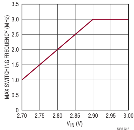
Max Programmable Switching Frequency vs Input Voltage
