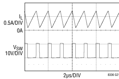
Switching Waveforms, Continuous Burst Mode Operation
