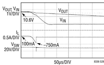
Waveforms, Reverse Current Protection in PassThru Mode
