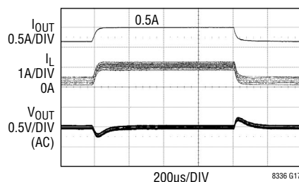
Switching Waveforms, Load Step in Pulse-Skipping Mode Operation
