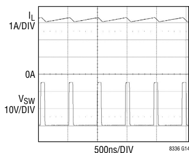
Switching Waveforms, Current Limit at 85% Duty Cycle
