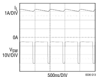
Switching Waveforms, Current Limit at 15% Duty Cycle
