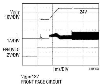
Switching Waveforms, Soft-Start
