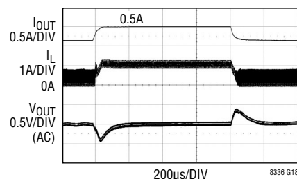
Switching Waveforms, Load Step in Burst Mode Operation
