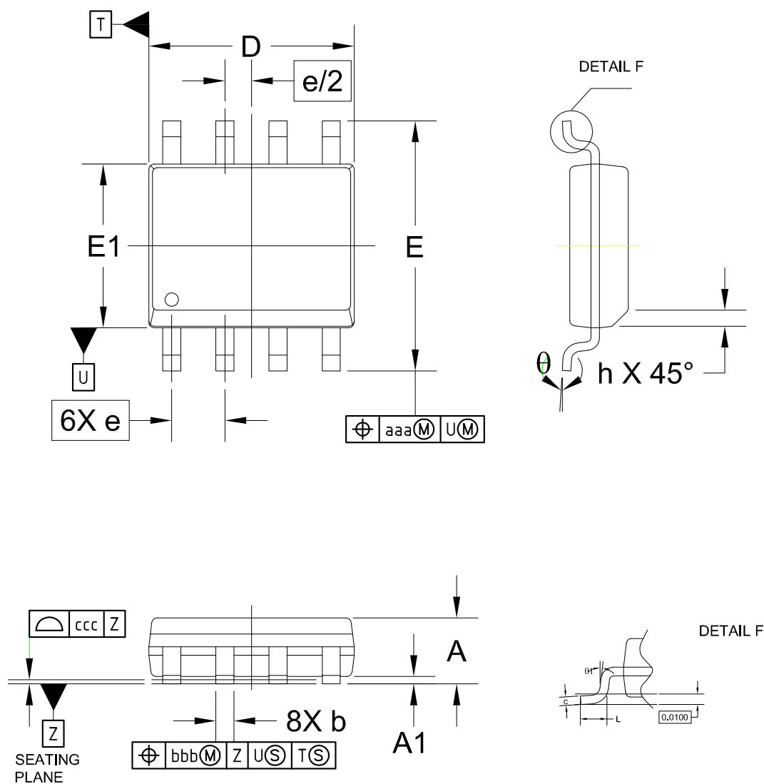
Figure 14. SO-8 package outline
