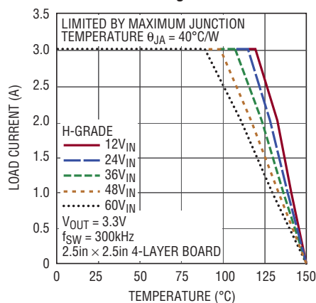
Thermal Derating
