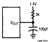
Load Circuit for t_{D0}
