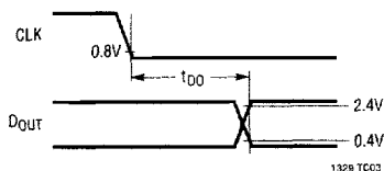
Voltage Waveforms for t_{D0}
