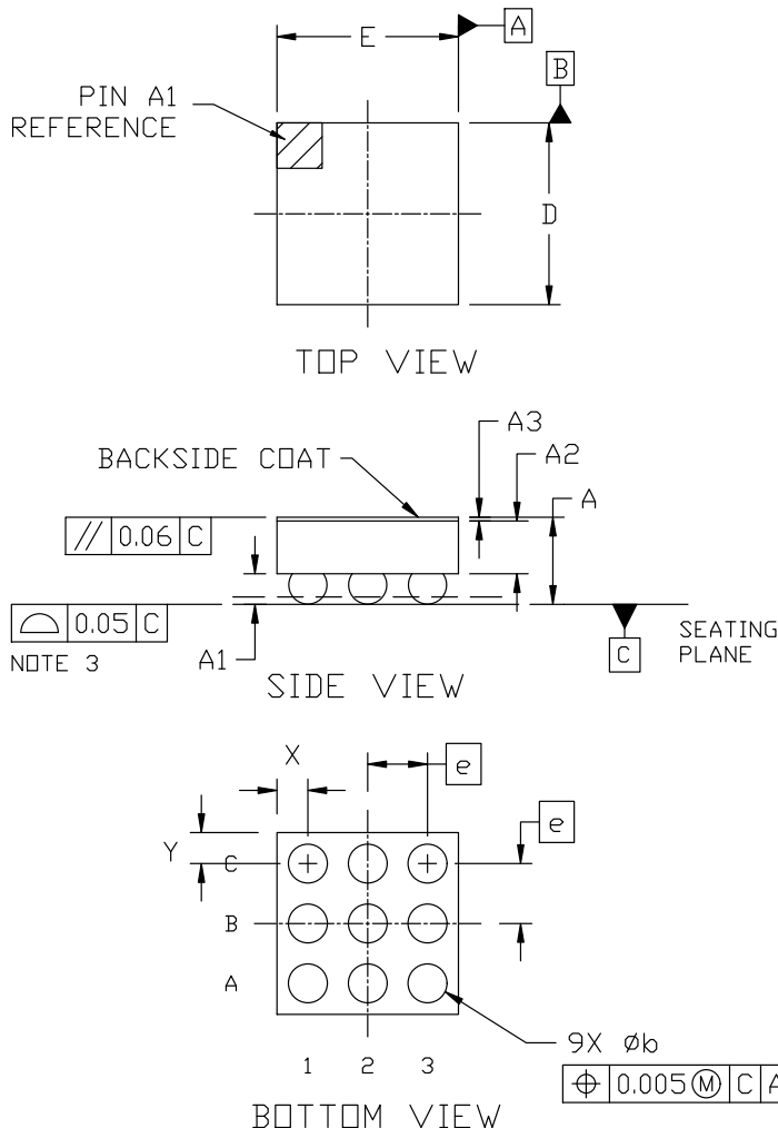
WLCSP9 1.215x1.215x0.581 CASE 567QW ISSUE A
