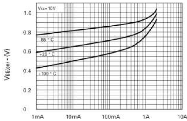
I_C -Collector Current V_{BE(on)} v I_C
