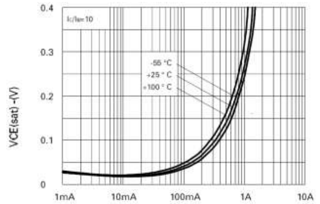
I_C -Collector Current V_{CE(sat)} v I_C
