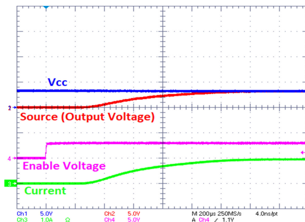
Figure 11. Slew Rate Control for NIS6432
