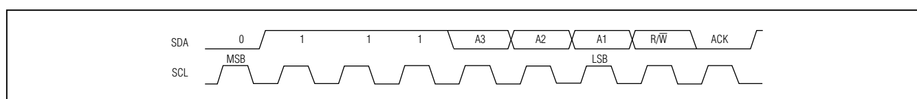
Figure 6. Slave Address
