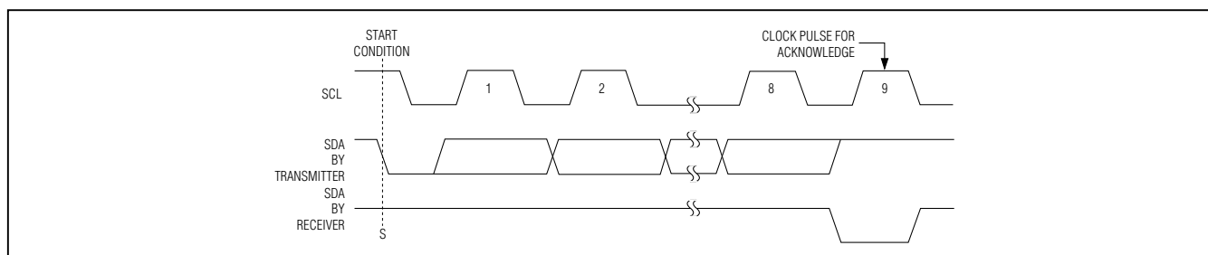
Figure 5. Acknowledge
