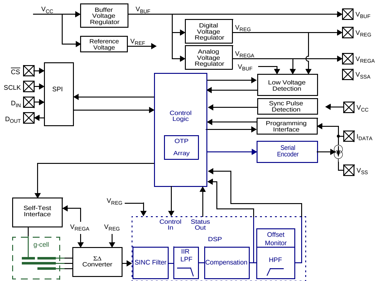
Figure 3. Block Diagram
