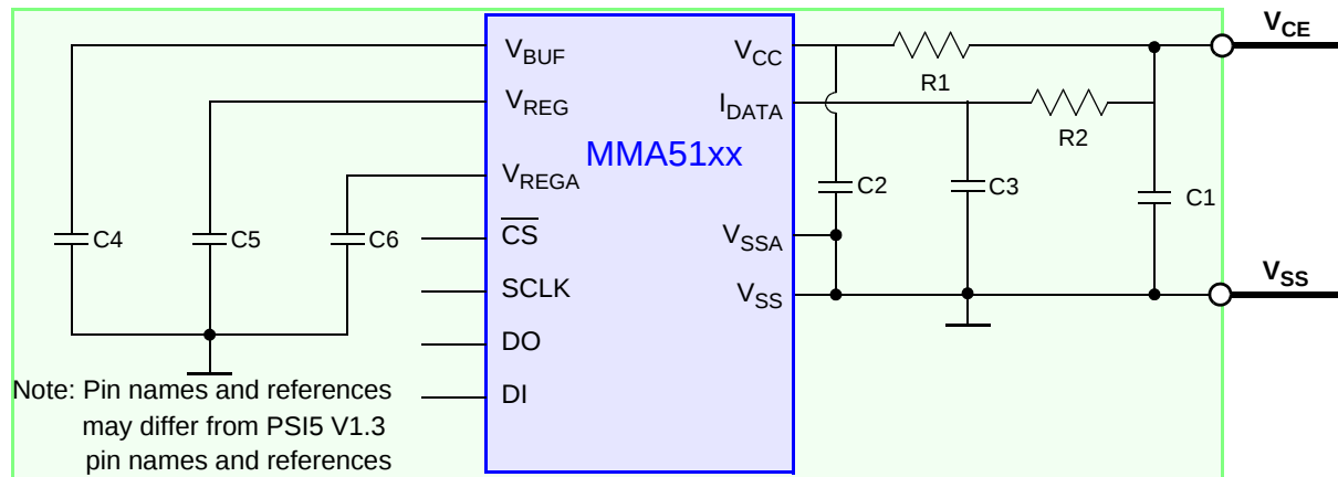
Figure 1. Application Diagram
