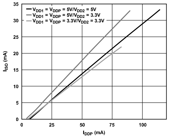
Figure 8. Isolated I_{SO} as a Function of External Load, No Dynamic Current Draw at 5 V/5 V, 5 V/3.3 V, and 3.3 V/3.3 V
