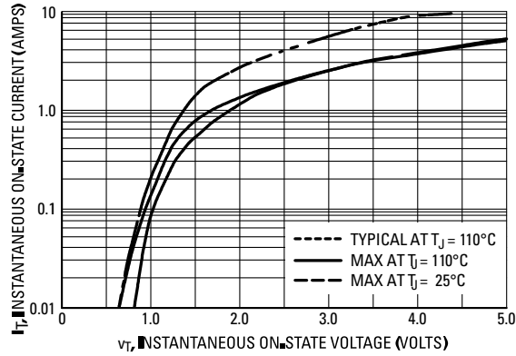
Figure 2. On-State Characteristics
