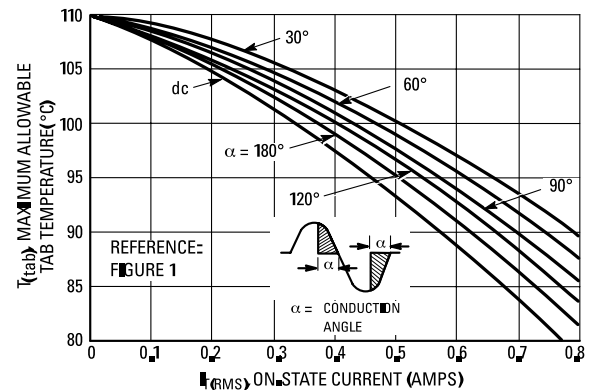
Figure 7. Current Derating Reference: MT2 Tab
