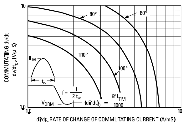
Figure 11. Typical Commutating dv/dt vs Current Crossing Rate and Junction Temperature
