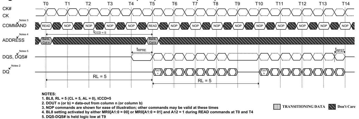
Figure 33. Nonconsecutive READ (BL8) to READ (BL8)
