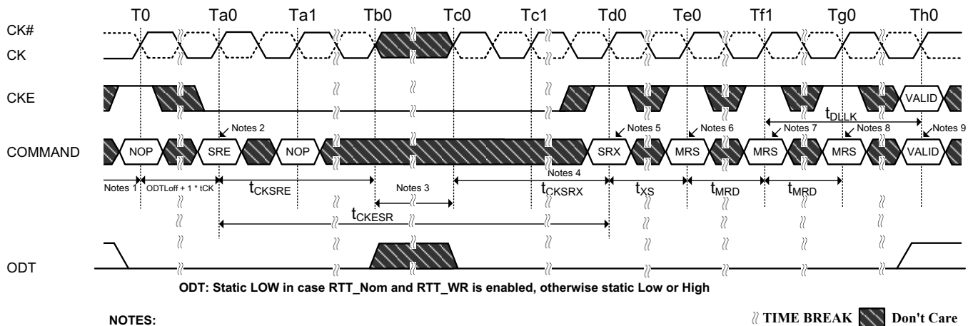
Figure 11. DLL Switch Sequence from DLL-off to DLL on
