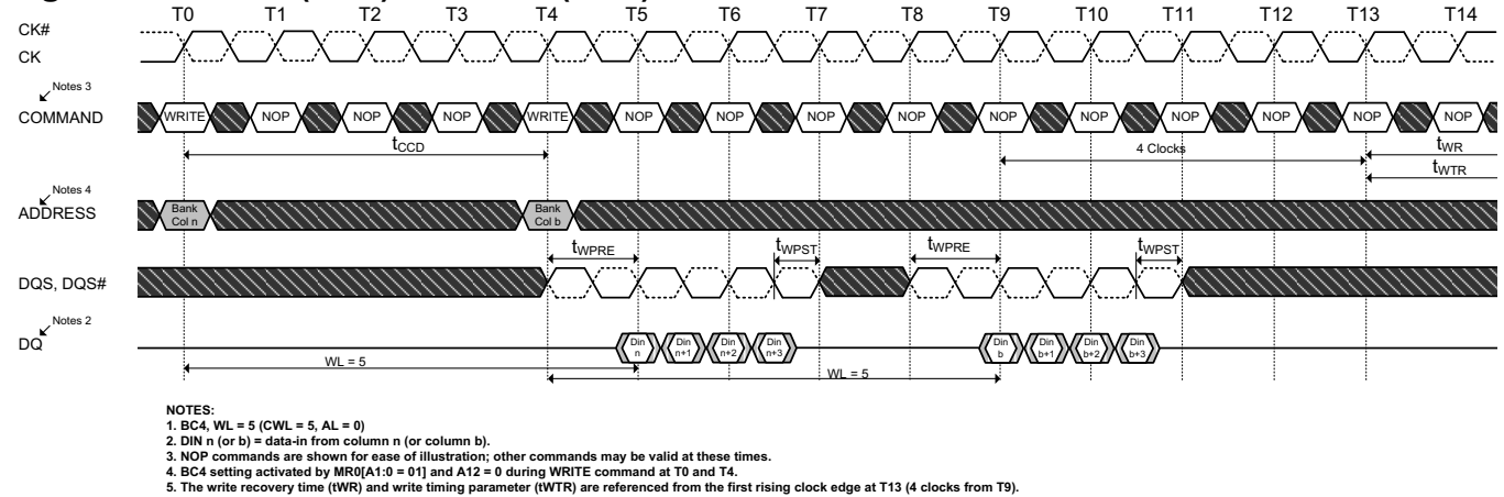
Figure 50. WRITE(BC4) to WRITE(BC4) OTF
