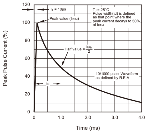
Fig.3 - Pulse Waveform
