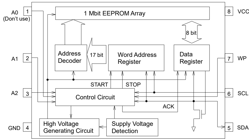
Figure 4. Block Diagram
