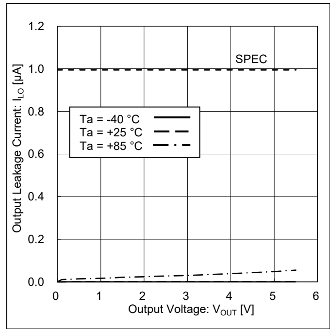
Figure 12. Output Leakage Current vs Output Voltage
