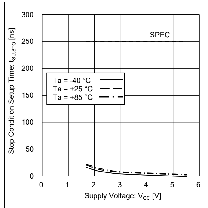
Figure 30. Stop Condition Setup Time vs Supply Voltage
