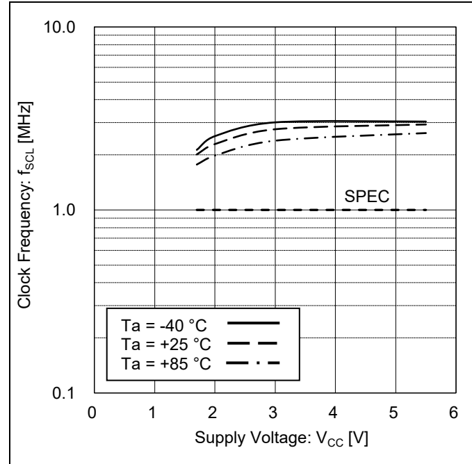
Figure 16. Clock Frequency vs Supply Voltage
