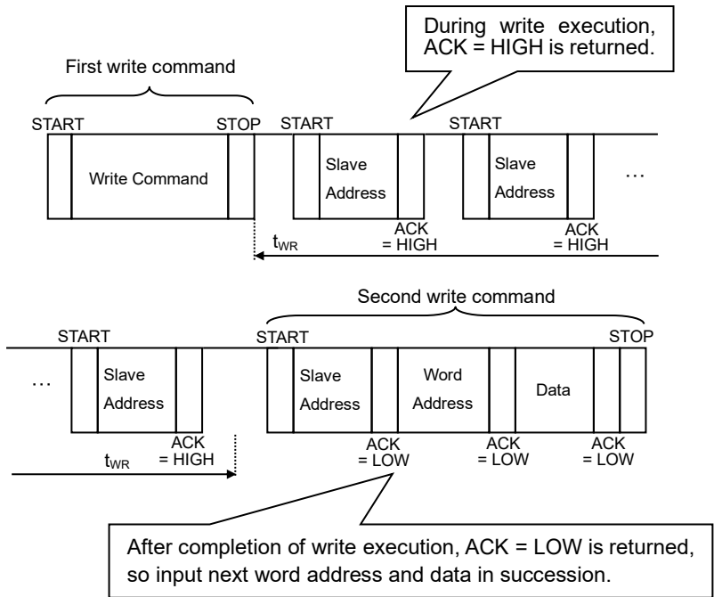
Figure 48. The Case of Continuous Write by Acknowledge Polling
