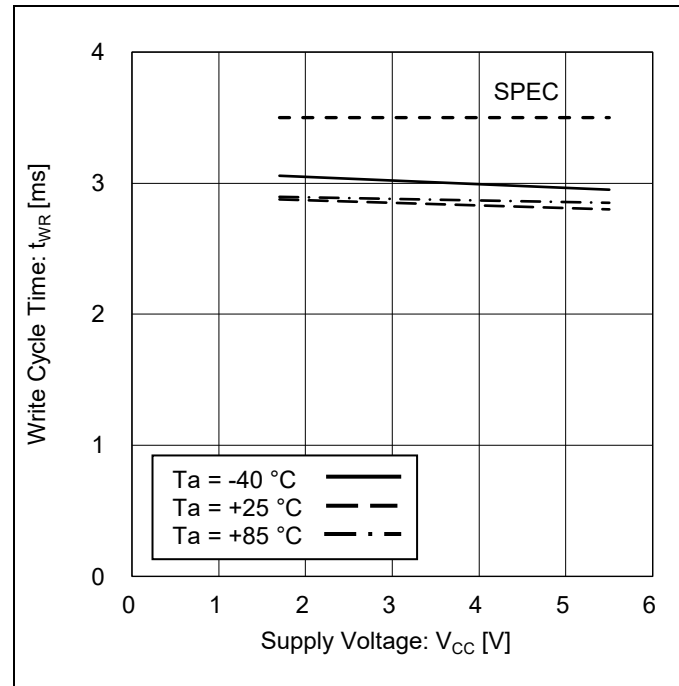
Figure 32. Write Cycle Time vs Supply Voltage
