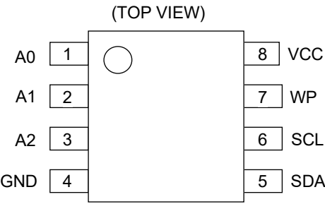
Figure 3. Pin Configuration
