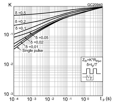
Figure 2. Thermal impedance
