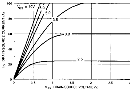
Figure 1. On-Region Characteristics.
