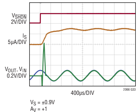
Enable Transient with Sinusoidal Input
