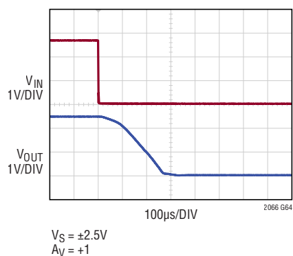
Positive Input Overload Recovery
