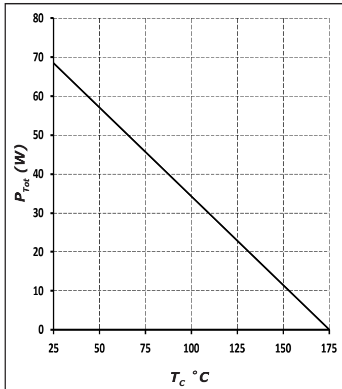
Figure 4. Power Derating
