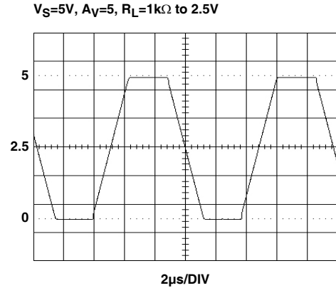
FIGURE 22. OUTPUT SWING
