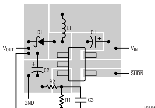
Figure 7. Suggested Layout
