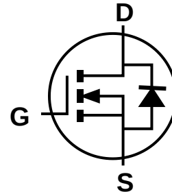
Internal Schematic
