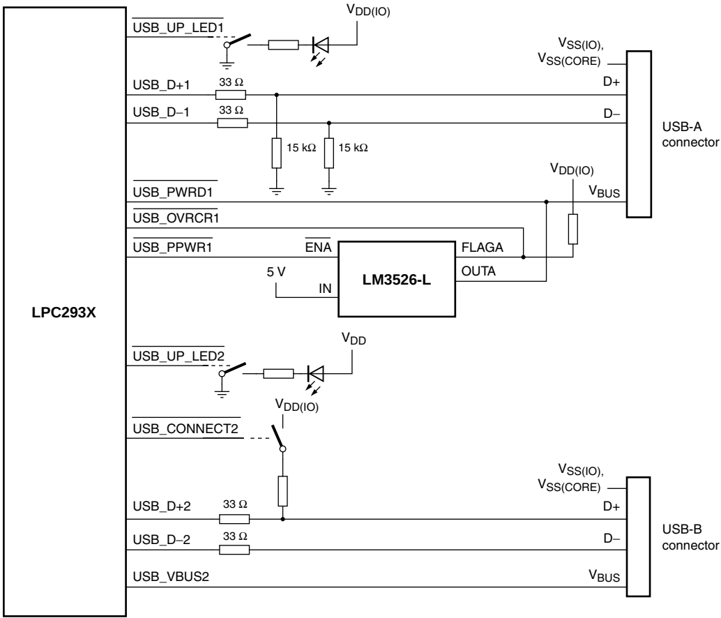
Fig 36. LPC2930 USB OTG port configuration: USB port 2 device, USB port 1 host
