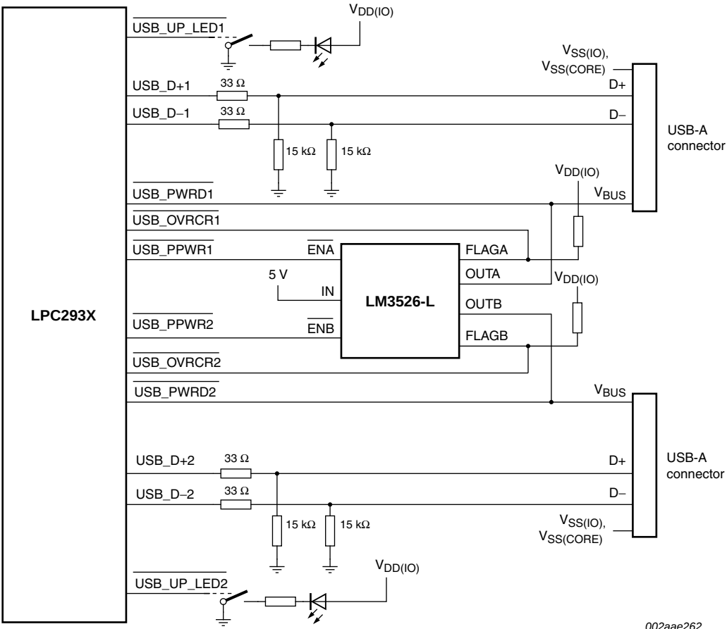
Fig 35. LPC2930 USB OTG port configuration: USB port 1 host, USB port 2 host
