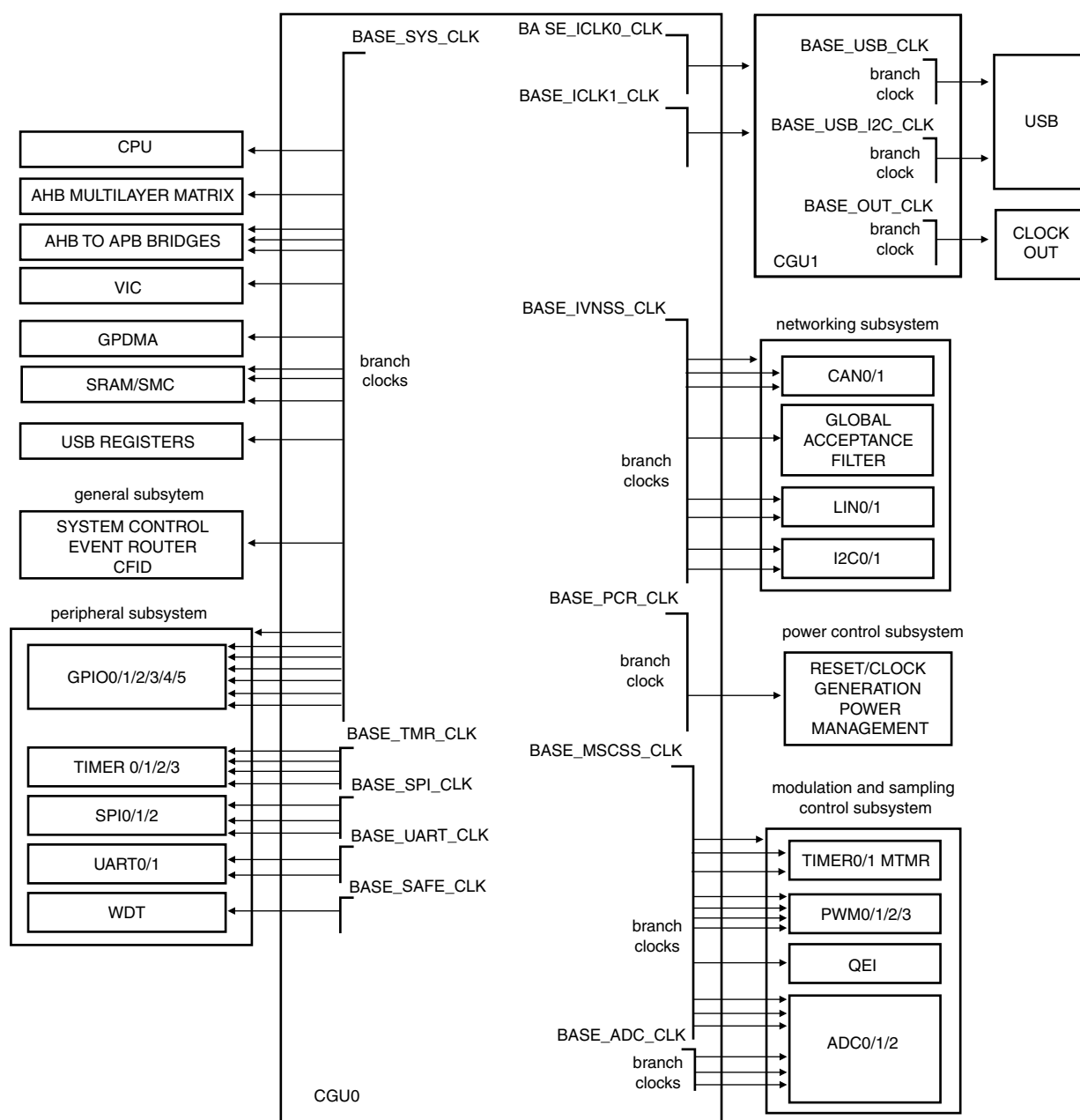
Fig 4. LPC2930 overview of clock areas
