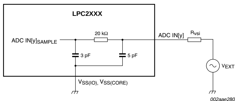
Fig 16. Suggested ADC interface - LPC2930 ADC1/2 IN[y] pin
