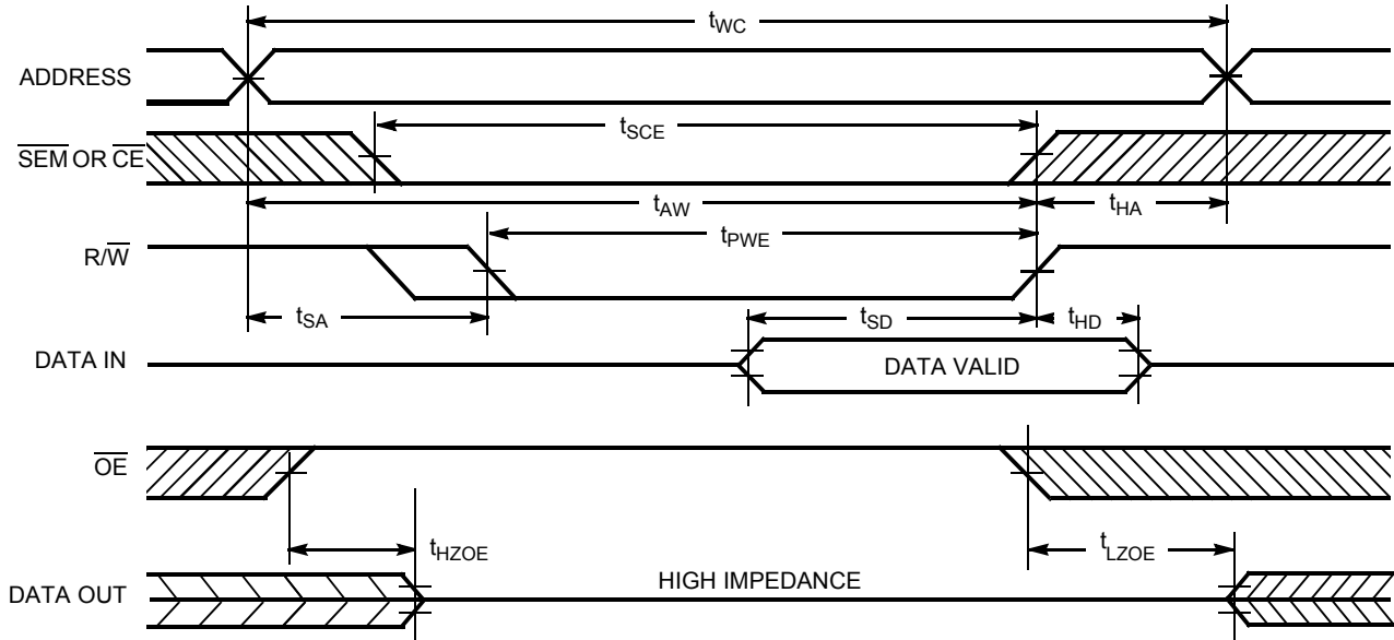
Figure 9. Write Cycle No. 2: \overline{R/W} Three-State Data I/Os (Either Port) [20, 22, 23]
