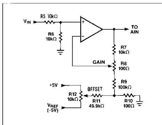
Figure 17. Offset (±20mV) and Gain (±0.5%) Trim Circuit
