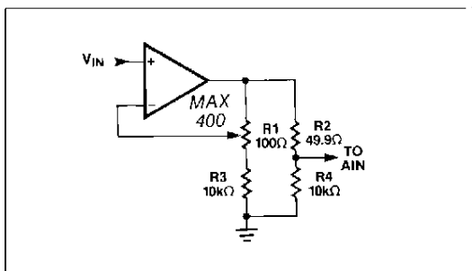
Figure 16. Trim Circuit for Gain Only (±0.5%)
