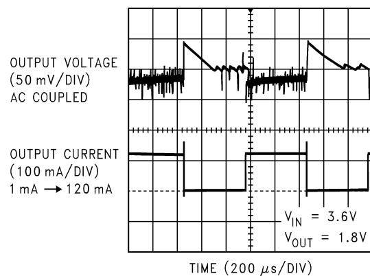
Transient Load Response
