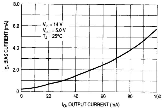
Figure 8. Bias Current versus Output Current
