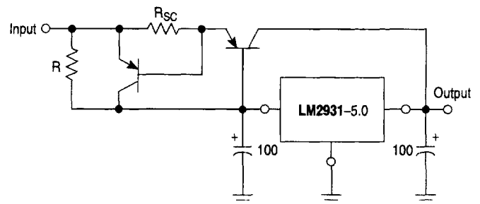
Figure 20. Current Boost Regulator with Short Circuit Projection
