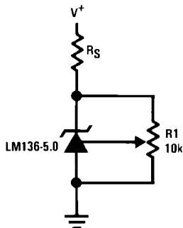
FIGURE 1. LM136-5.0 with Pot for Adjustment of
