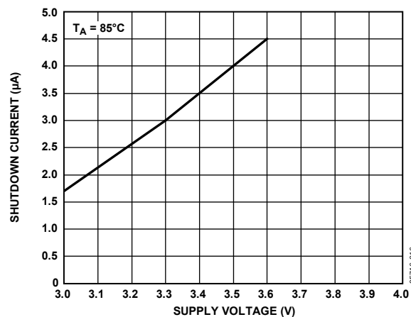
Figure 8. Shutdown Current vs. Supply Voltage
