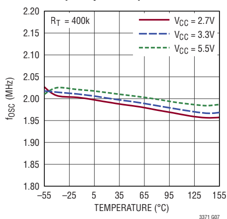
R_T Programmed Oscillator Frequency vs Temperature
