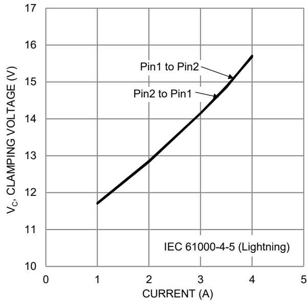
Figure 9 8x20 Clamping Voltage Characteristic
