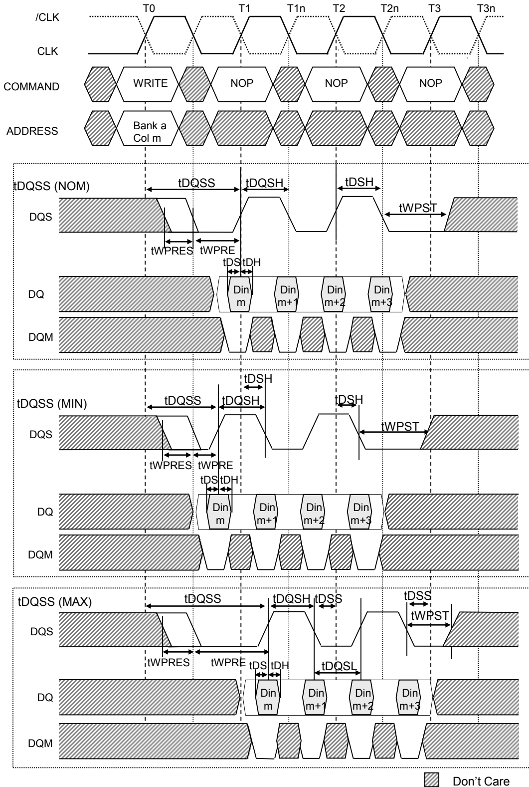
Figure 15: WRITE Operation
