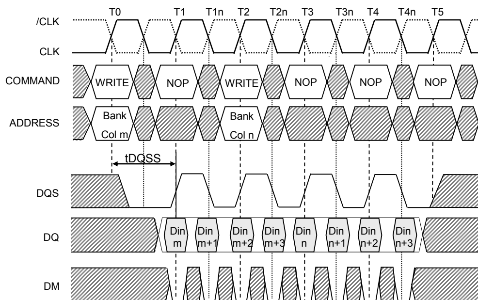
Figure 16: Consecutive WRITE-to-WRITE
