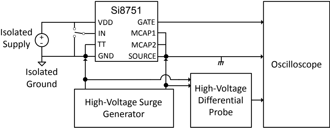
Figure 4.1. Common-Mode Transient Immunity Test Circuit
