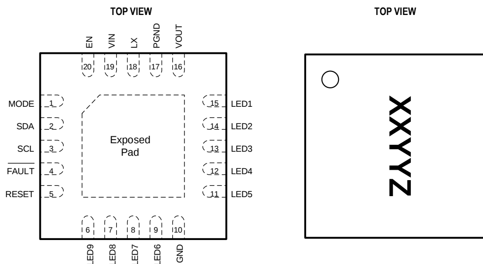
UQFN33-20
