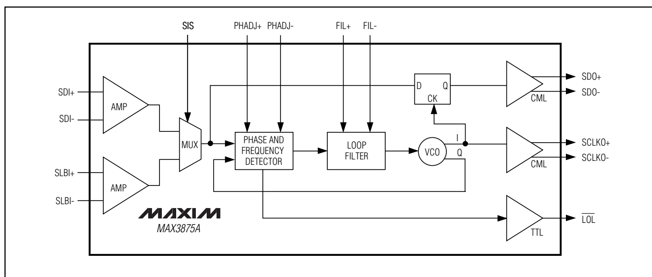
Figure 3. Functional Diagram
