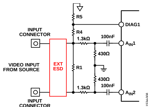
Figure 11. Diagnostic Connections
