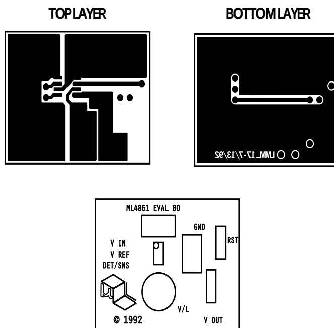
Figure 6. Sample PC Board Layout.
