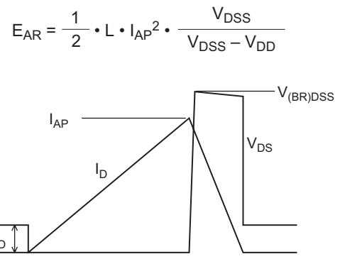
Avalanche Waveform
