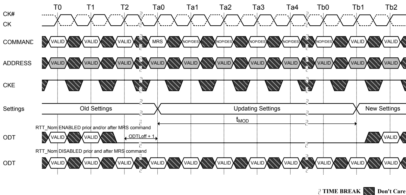
Figure 7. t_{MOD} timing
