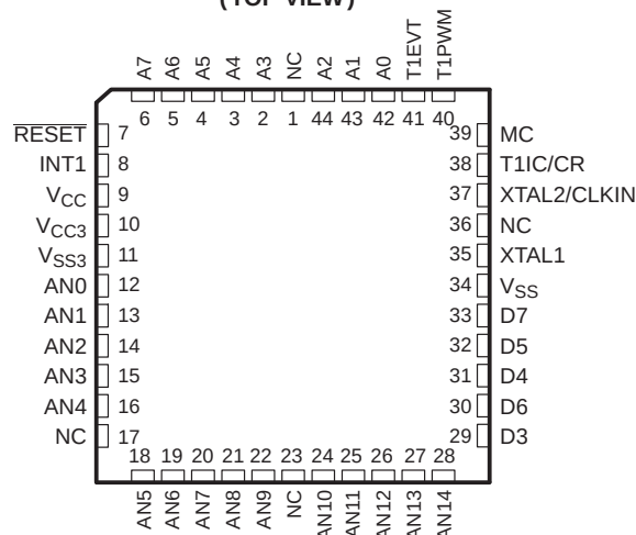
JC AND NJ PACKAGES (TOP VIEW)
