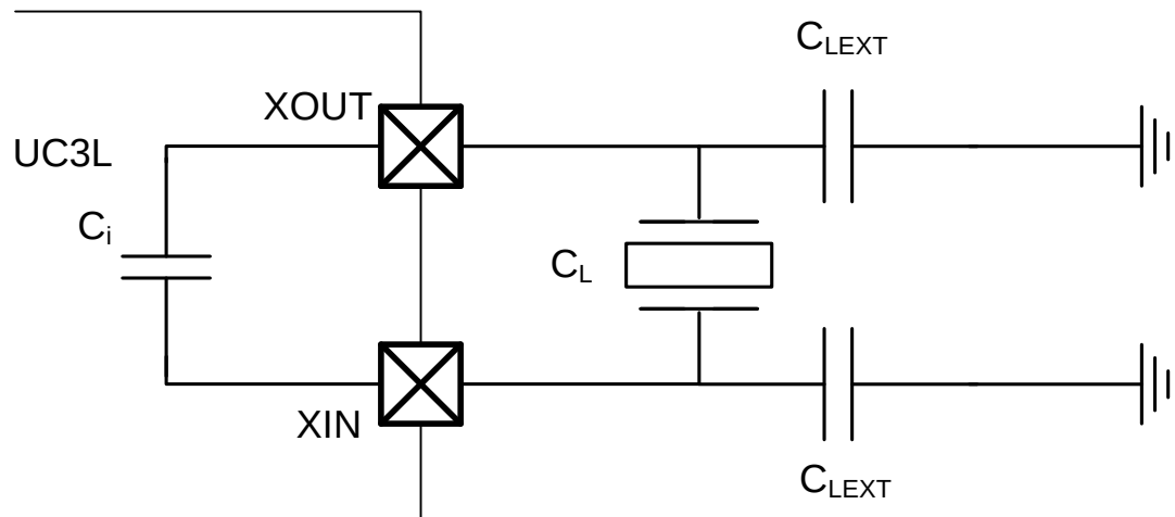
Figure 35-3. Oscillator Connection
