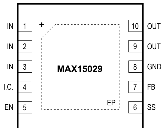
TDFN (3mm x 3mm)
