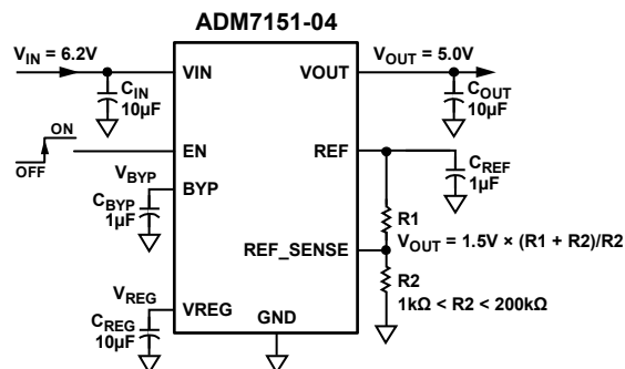
Figure 1. ADM7151-04 with V_{\text{OUT}} = 5\text{ V}
