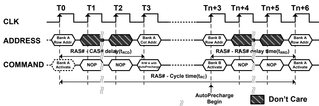
Figure 3. BankActivate Command Cycle (Burst Length = n)
