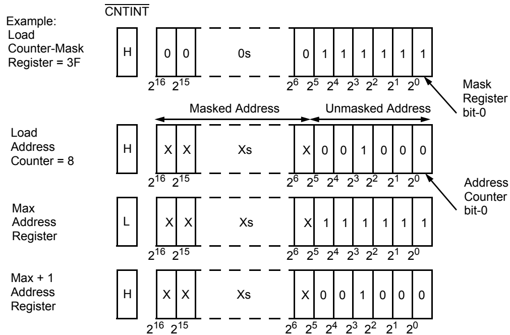
Figure 5. Programmable Counter-Mask Register Operation [1, 12]
