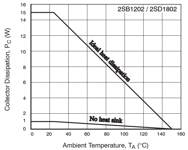
Figure 18. P_C - T_A
