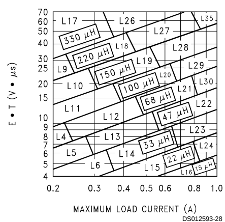
FIGURE 7. LM2598-ADJ
