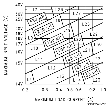
FIGURE 6. LM2598-12
