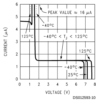
Shutdown/Soft-start Current
