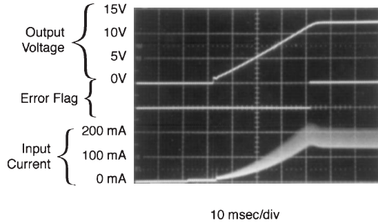
FIGURE 24. Output Voltage, Input Current, Error Flag Signal, at Start-Up, WITH Soft-start
