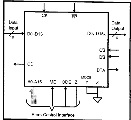
Fig. 3 - Data Memory Modes 1 and 2 Pinout
