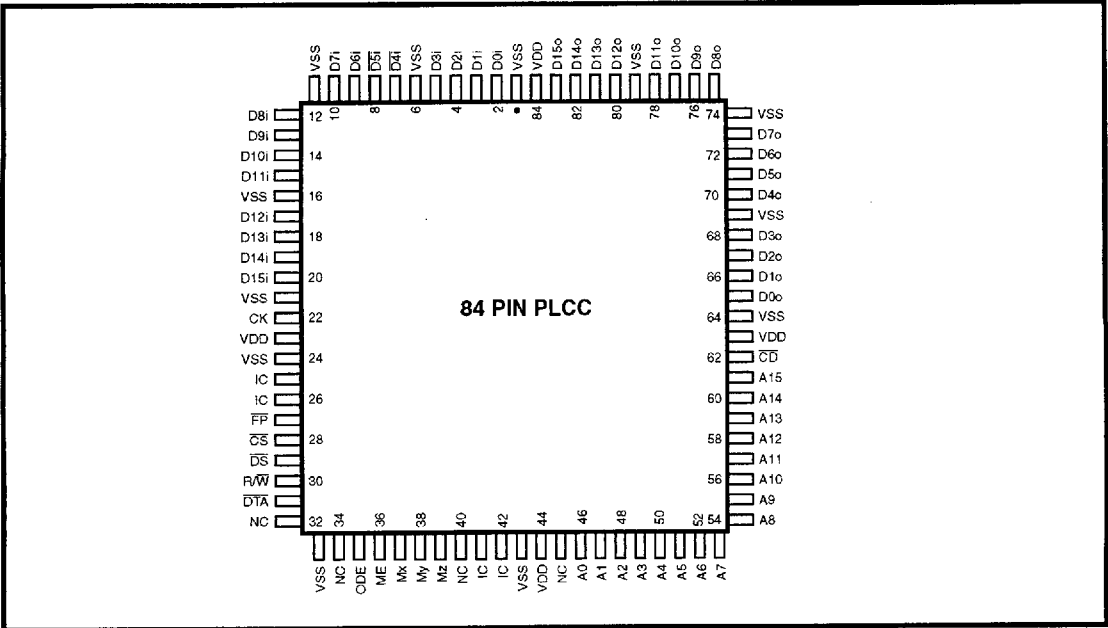
Figure 2 - Pin Connections
