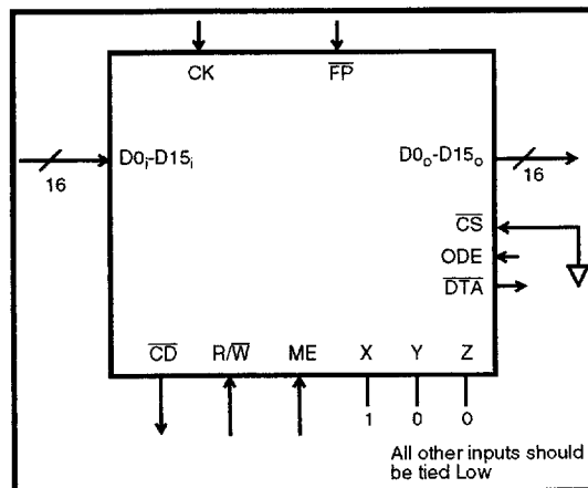
Fig. 10 - Counter Mode Pinout
