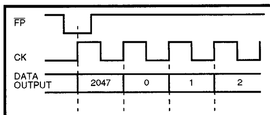
Fig. 9 - Connect Memory Mode-2 Functional Timing
